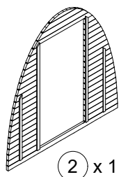
POD2.4-GS-DA1040x1870
